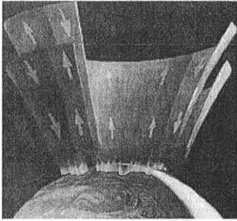
Fig. 2. Artists depiction of Birkeland currents flowing into and out of the earth's atmosphere at high latitude. These currents, once the subject of intense debate, are routinely measured by today's satellites and have total magnitudes of millions of amperes (megaamperes). Courtesy of S. G. Smith, Applied Physics Laboratory, The Johns Hopkins University.
