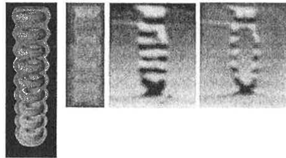
Fig. 8. Inner toroids within the stack of spheroids produced in a multi-megaampere plasma column. (a) Basic geometry. (b) Centimeter-size 1.3-MA pinch. (c) Centimeter-size 6-MA pinch. (d) Centimeter-size 6-MA pinch with optically dense (brightest) plasma shown.
