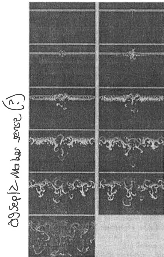
Fig. 11. Time evolution of an ionospheric layer shocked by Mach 1.2 pulse. Time increases from left to right and top to bottom. (RAGE calculation, R. Weaver, Los Alamos National Laboratory.)
